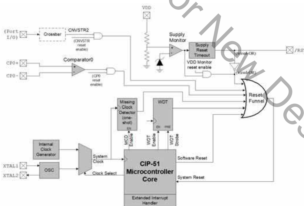
Figure 14.1. Reset Sources
