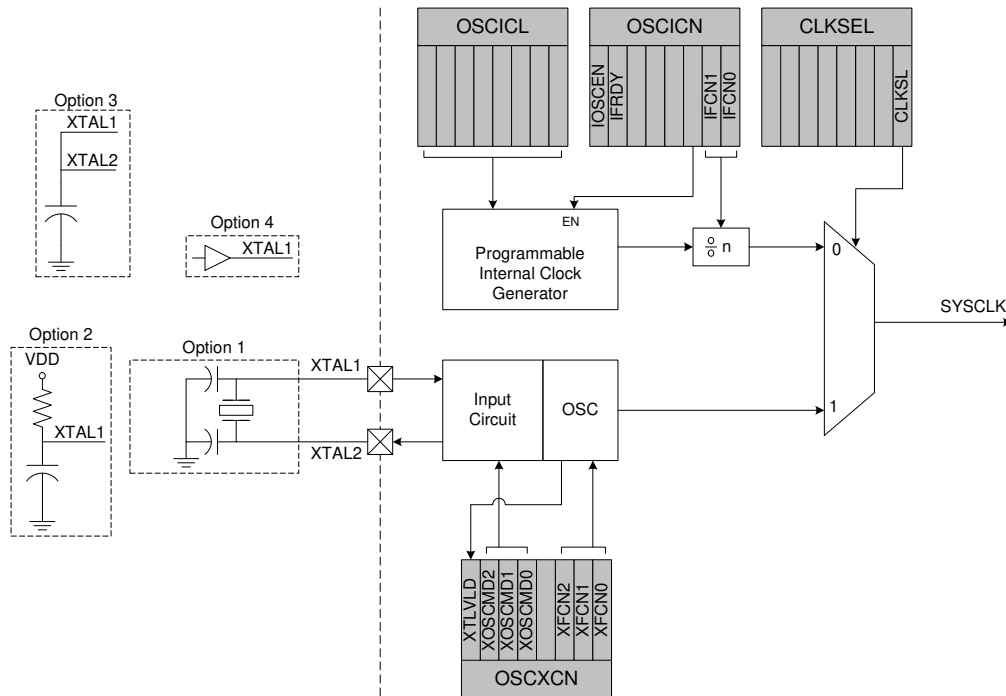
Figure 15.1. Oscillator Diagram
