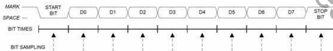
Figure 23.4. 8-Bit UART Timing Diagram
