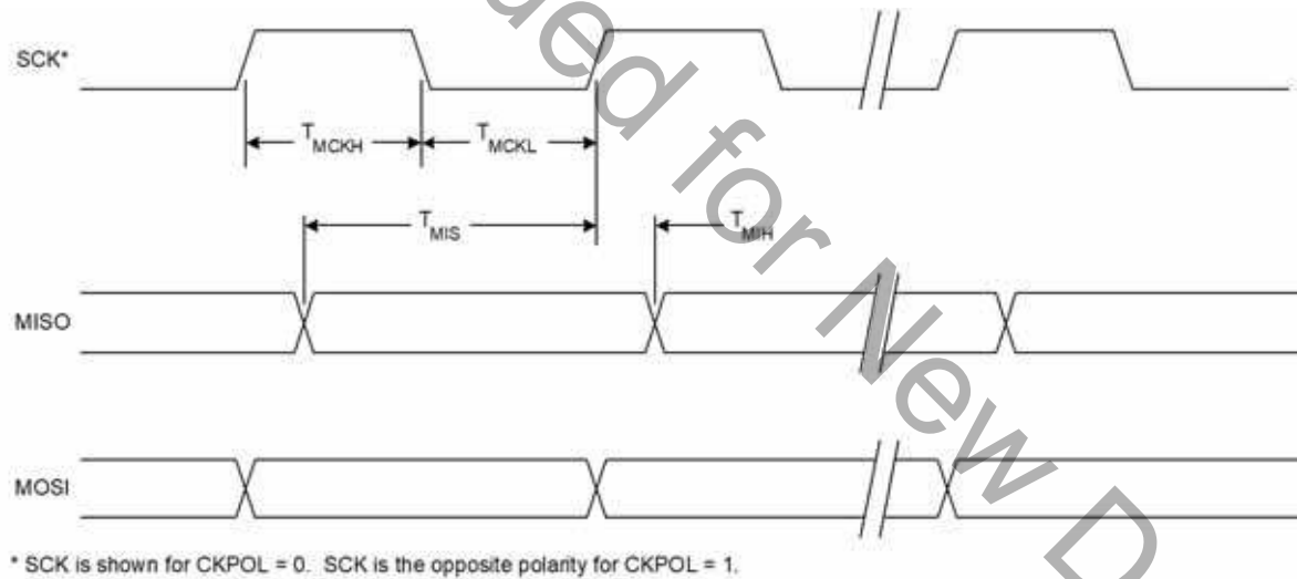
Figure 21.13. SPI Master Timing (CKPHA = 1)
