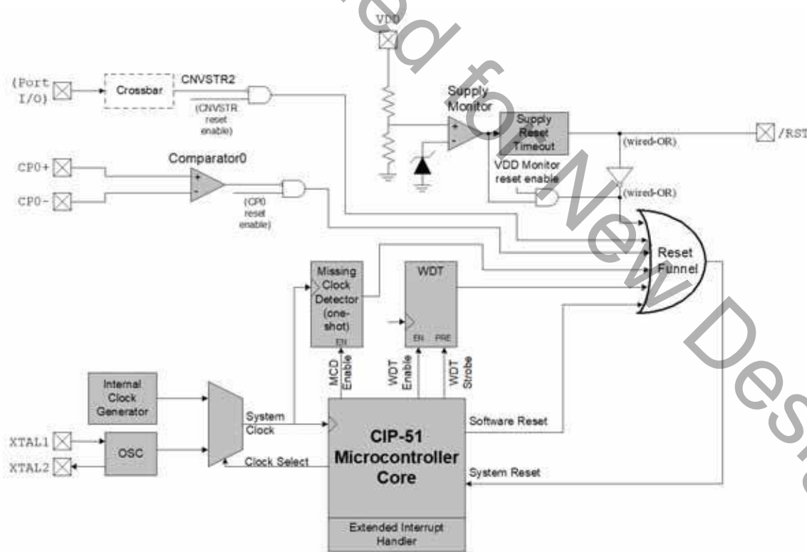
Figure 1.6. On-Board Clock and Reset
