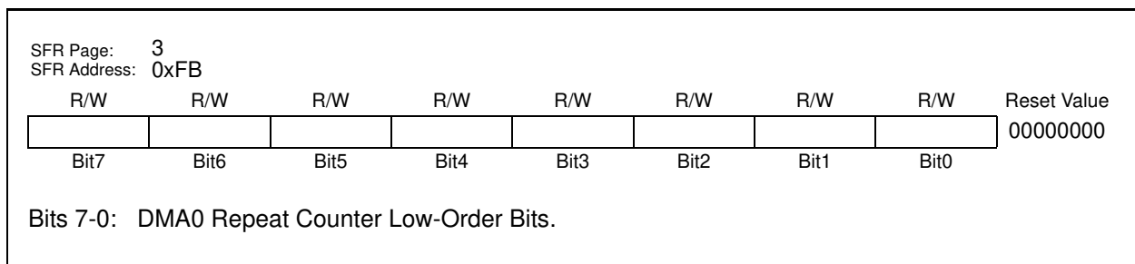
Figure 6.17. DMA0CSL: DMA0 Repeat Counter LSB Register
