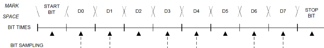
Figure 22.4. 8-Bit UART Timing Diagram
