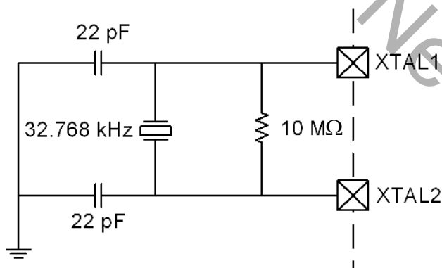
Figure 14.2. 32.768 kHz External Crystal Example
