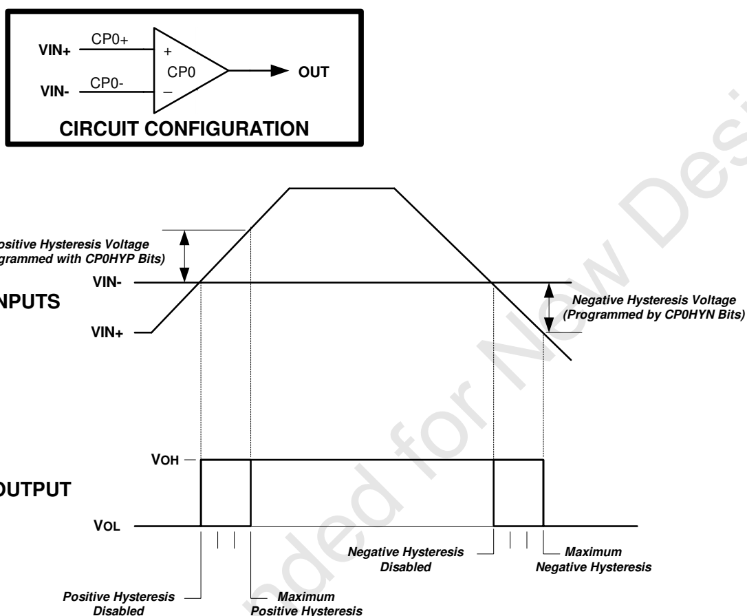
Figure 11.2. Comparator Hysteresis Plot
