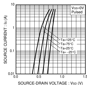
Fig.9 Source Current vs. Source-Drain Voltage
