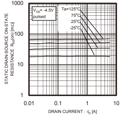
Fig.3 Static Drain-Source On-State Resistance vs. Drain Current (2)
