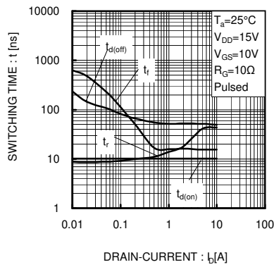
Fig.11 Switching Characteristics
