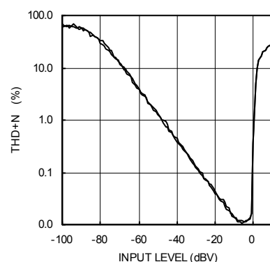
Fig.23 Speaker Preamp Total Harmonic Distortion (SPOL / SPOR)
