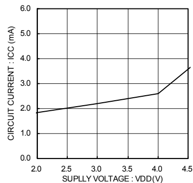
Fig.3 Headphone Amplifier Operation Current
