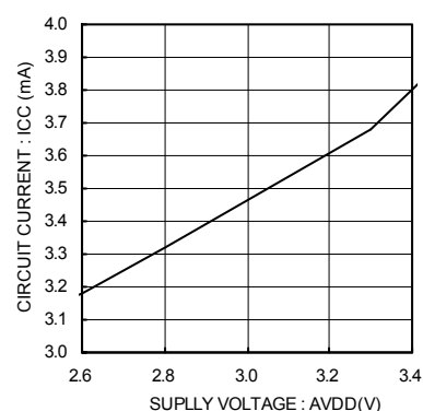
Fig.17 AVDD Operation Current (digital melody)
