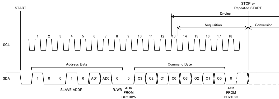
Figure 1. Write Protocol
