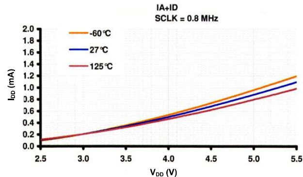
Figure 1. I_{DD} vs V_{DD} ( f_{SCLK}=0.8MHz )
