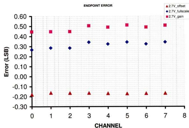
Figure 3. ENDPOINT ERROR vs CHANNEL ( V_{DD}=2.7V )
