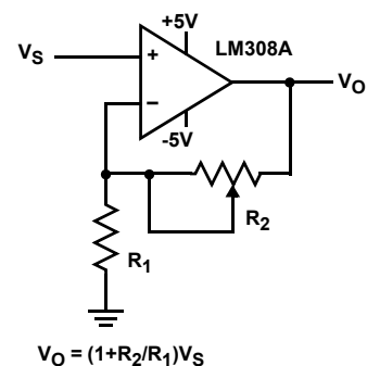
NONINVERTING AMPLIFIER
