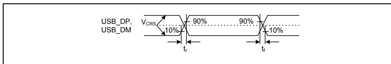
Figure 2.77 USB_DP and USB_DM output timing
