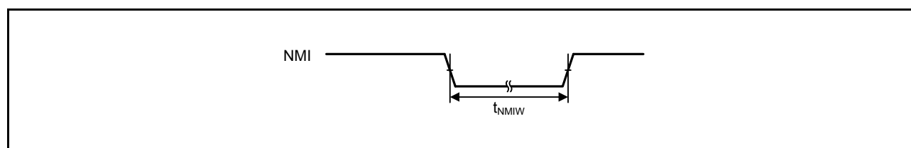
Figure 2.38 NMI interrupt input timing
