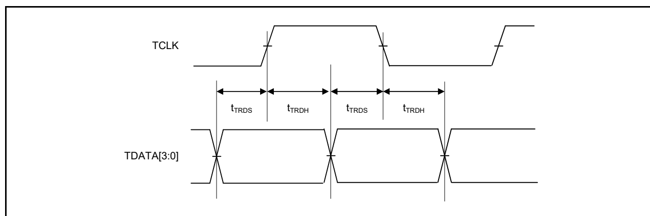
Figure 2.58 ETM output timing
