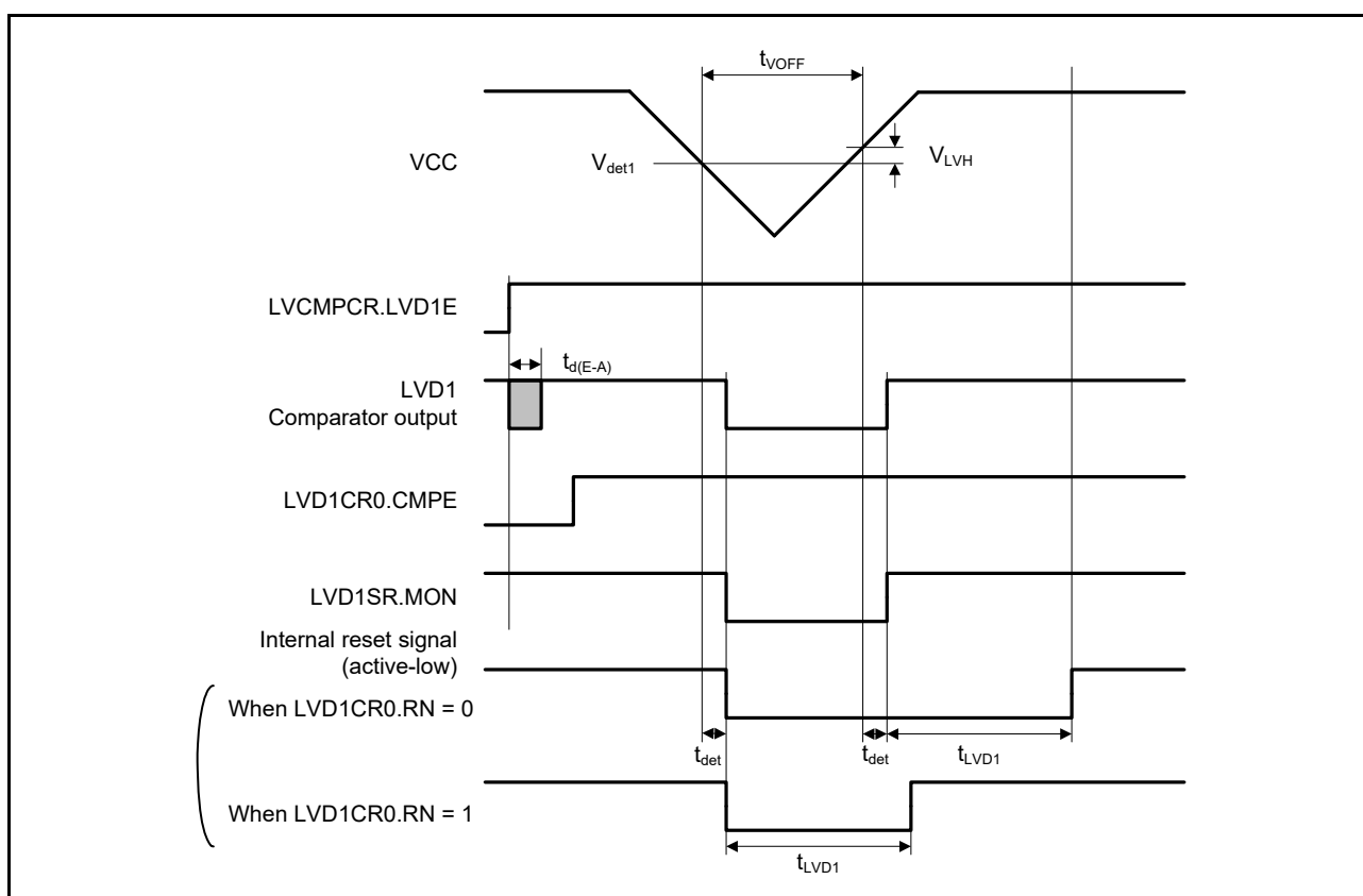
Figure 2.47 Voltage detection circuit timing (V det1 )
