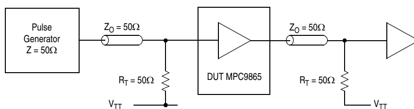
Figure 4. MPC9865 AC Test Reference (LVCMOS Outputs)
