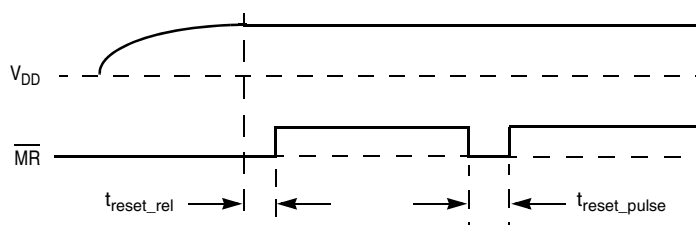
Figure 2. \overline{MR} Operation
