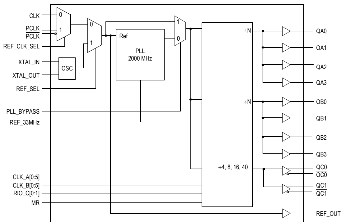
Figure 1. MPC9850 Logic Diagram
