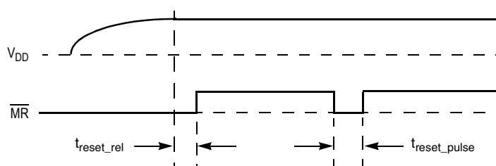
Figure 2. \overline{MR} Operation
