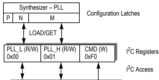
Figure 3. I²C Mode Register Set
