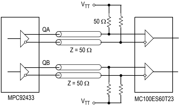
Figure 13. Interfacing with LVCMOS Logic for f < 300\text{ MHz}
