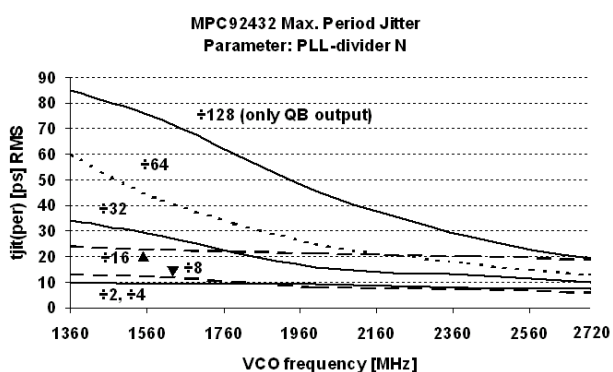
Figure 9. MPC92432 Period Jitter
