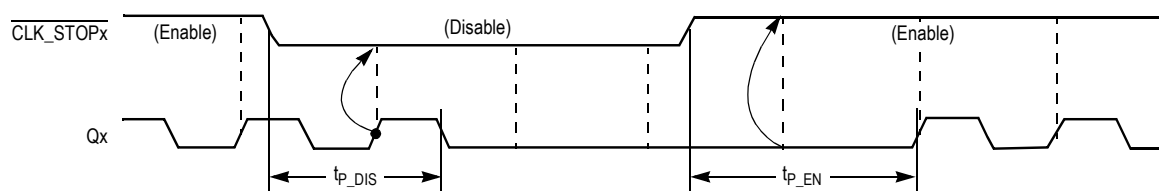
Figure 5. Clock Stop Timing for NB = 0 ( f_{\text{QA}} = f_{\text{QB}} )
