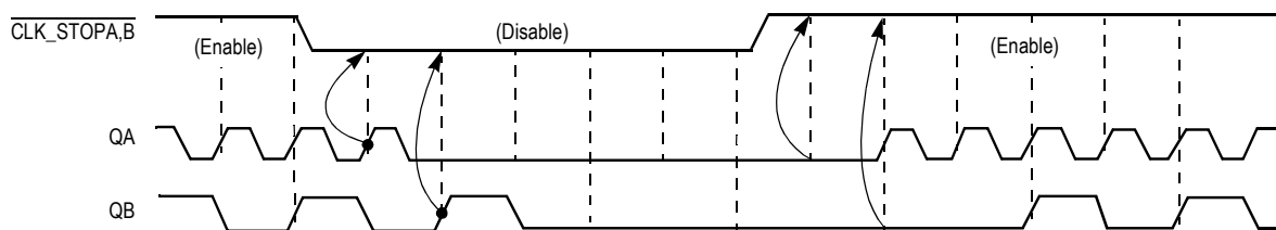
Figure 6. Clock Stop Timing for NB = 1 ( f_{\text{QA}} = 2 f_{\text{QB}} )
