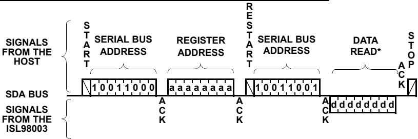
FIGURE 7. CONFIGURATION REGISTER READ
