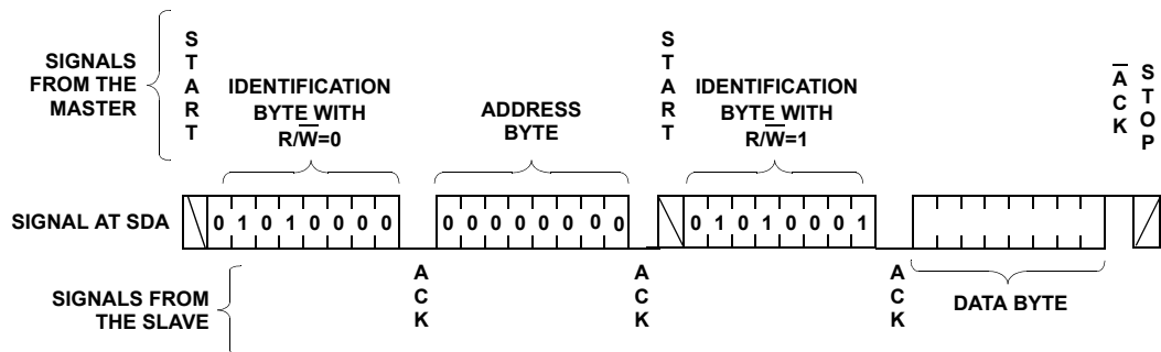
FIGURE 18. READ SEQUENCE
