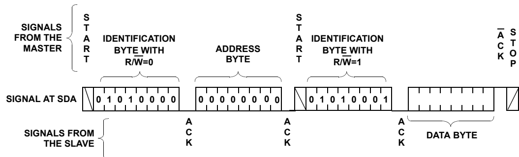
FIGURE 18. READ SEQUENCE
