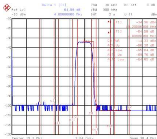
FIGURE 7. UMTS AT 19.2MHz, 76.8MSPS (65dB 1stACPR, 64dB 2ndACPR)
