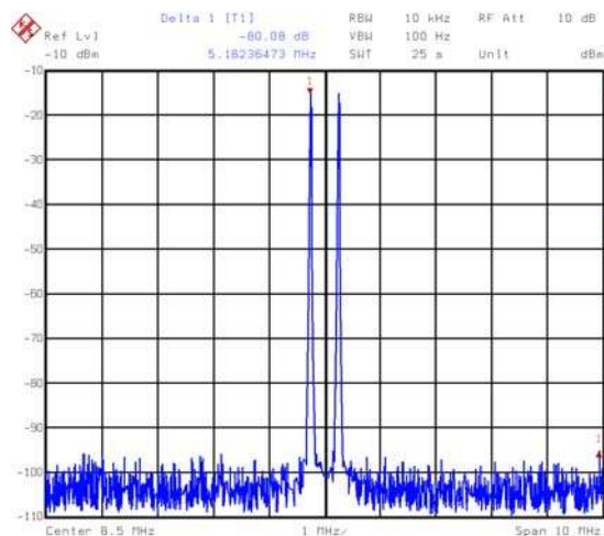
FIGURE 11. TWO TONES (CF=6) AT 8.5MHz, 50MSPS CLOCK, 500kHz SPACING (80dBc - 10MHz WINDOW, 6dB PAD)
