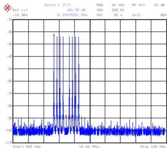
FIGURE 10. EIGHT TONES (CREST FACTOR=8.9) AT 37MHz, 210MSPS CLOCK, 2.1MHz SPACING (64dBc - NYQUIST)
