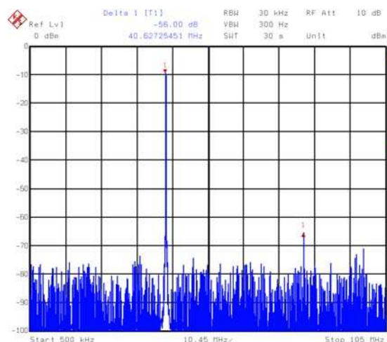
FIGURE 2. ONE TONE AT 40.4MHz, 210MSPS CLOCK (56dBc - NYQUIST, 6dB PAD)
