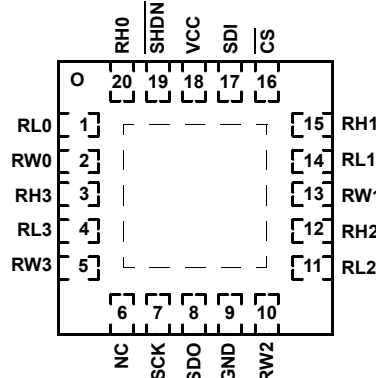
ISL22446 (20 LD TQFN) TOP VIEW
