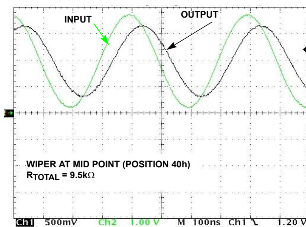
FIGURE 12. FREQUENCY RESPONSE (2.6MHz)
