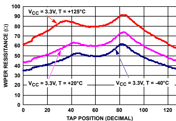
FIGURE 1. WIPER RESISTANCE vs TAP POSITION [ I(\text{RW}) = V_{\text{CC}}/R_{\text{TOTAL}} ] FOR 10k \Omega (W)
