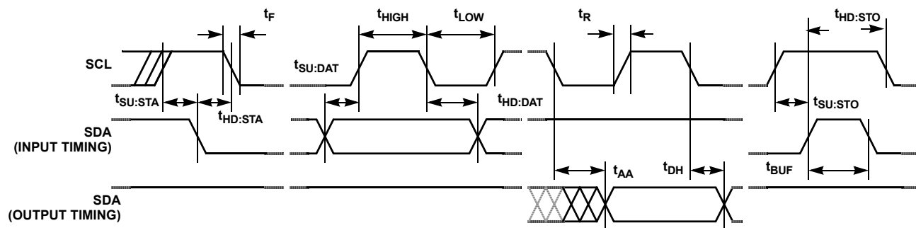
FIGURE 1. BUS TIMING
