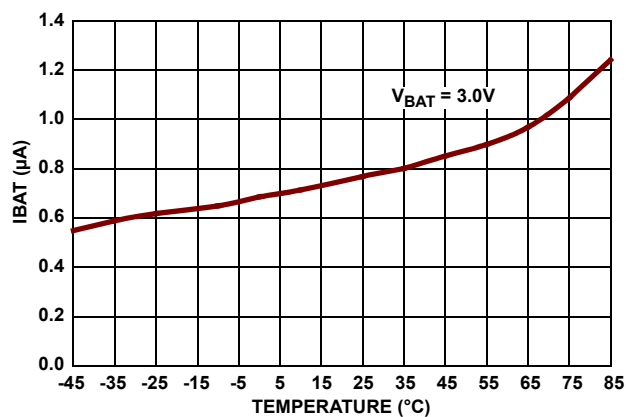
FIGURE 8. I_{BAT} vs TEMPERATURE
