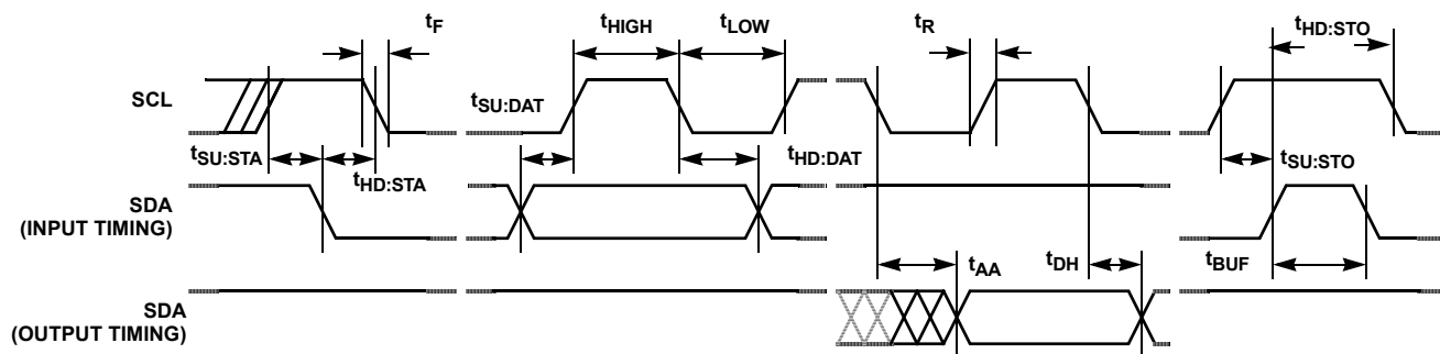
FIGURE 1. BUS TIMING
