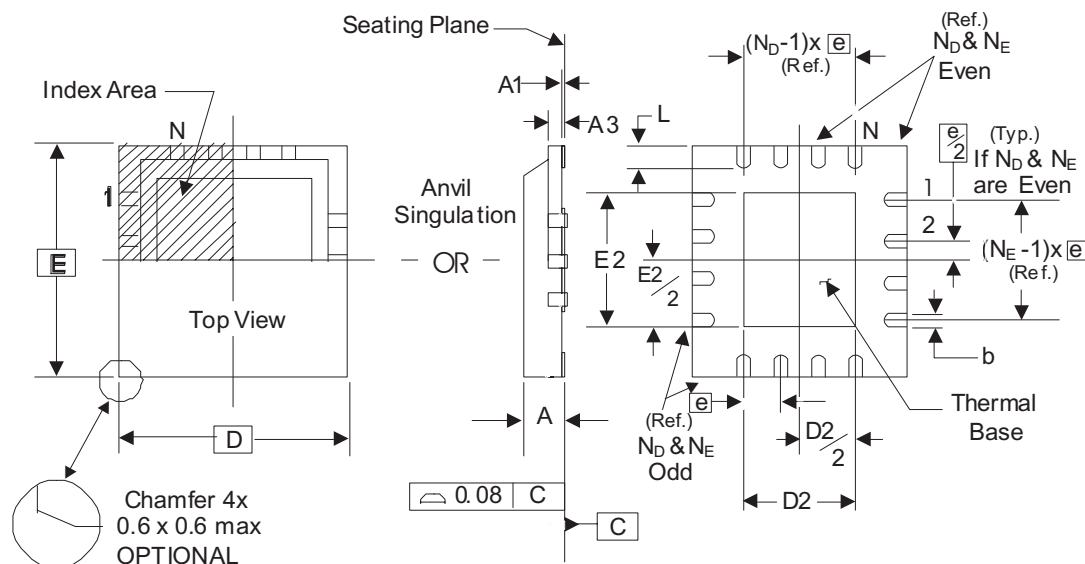
All Dimensions in Millimeters Symbol Minimum Maximum N 16 A 0.80 1.0 A1 0 0.05 A3 0.25 Reference b 0.18 0.30 e 0.50 Basic D, E 3.0 D2, E2 1.00 1.80 L 0.30 0.50 N D N E 4.0
