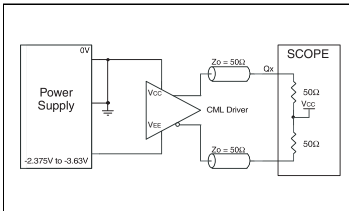
Open Collector Output Load AC Test Circuit
