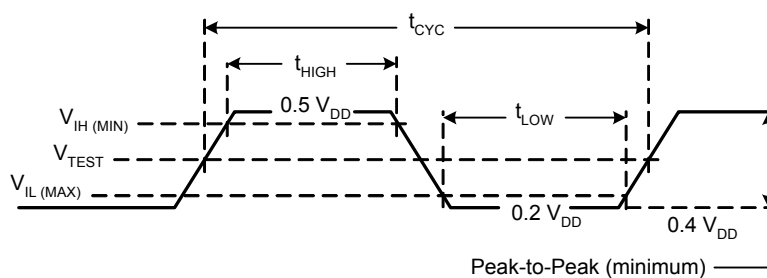
Figure 4. Clock Waveform
