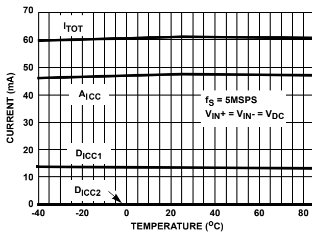
FIGURE 12. POWER SUPPLY CURRENT vs TEMPERATURE
