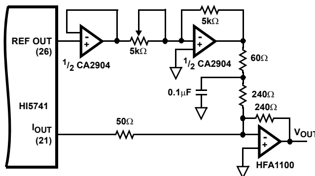
FIGURE 26. BIPOLAR OUTPUT CONFIGURATION
