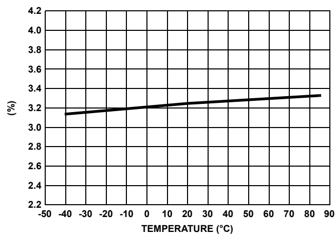
FIGURE 9. TYPICAL GAIN ERROR OVER TEMPERATURE
