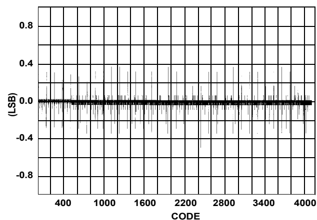
FIGURE 7. TYPICAL DNL
