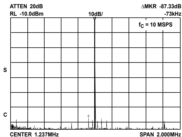
FIGURE 9. SPURIOUS FREE DYNAMIC RANGE = 87.3dBc
