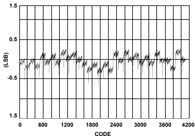
FIGURE 6. TYPICAL INL
