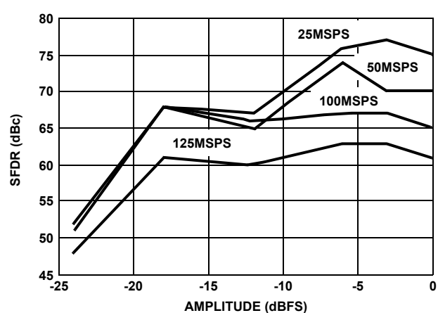
FIGURE 6. SFDR vs AMPLITUDE, f_{CLK}/f_{OUT} = 10
