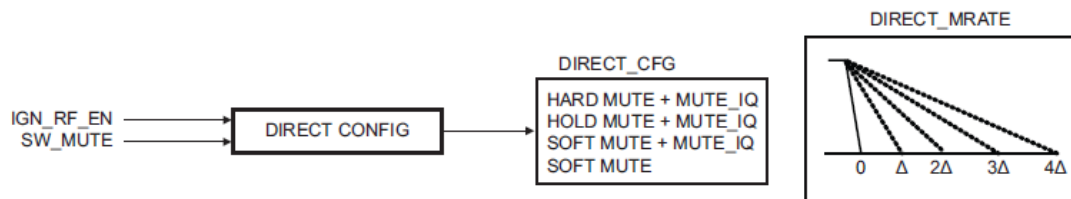
Fig 56. RF_ENABLE trigger in MUTE controller
