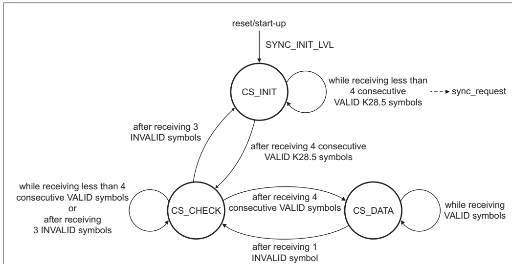
Fig 78. Code group synchronization
