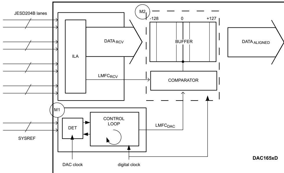
Fig 68. Modules of MDS implementation
