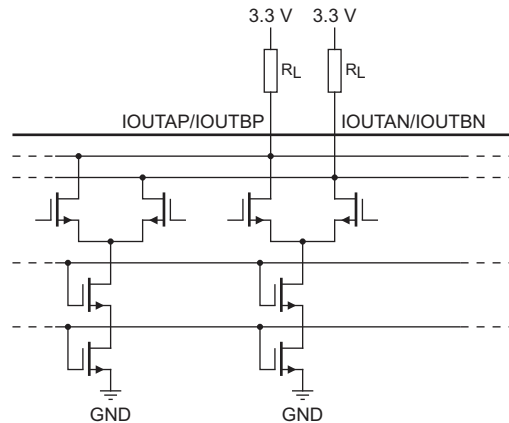
Fig 61. Equivalent analog output circuit
