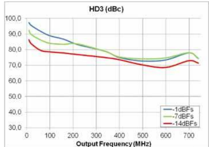
Fig 7. HD3 (dBc) over Nyquist depending of f out (MHz) and input level (dBFS)
