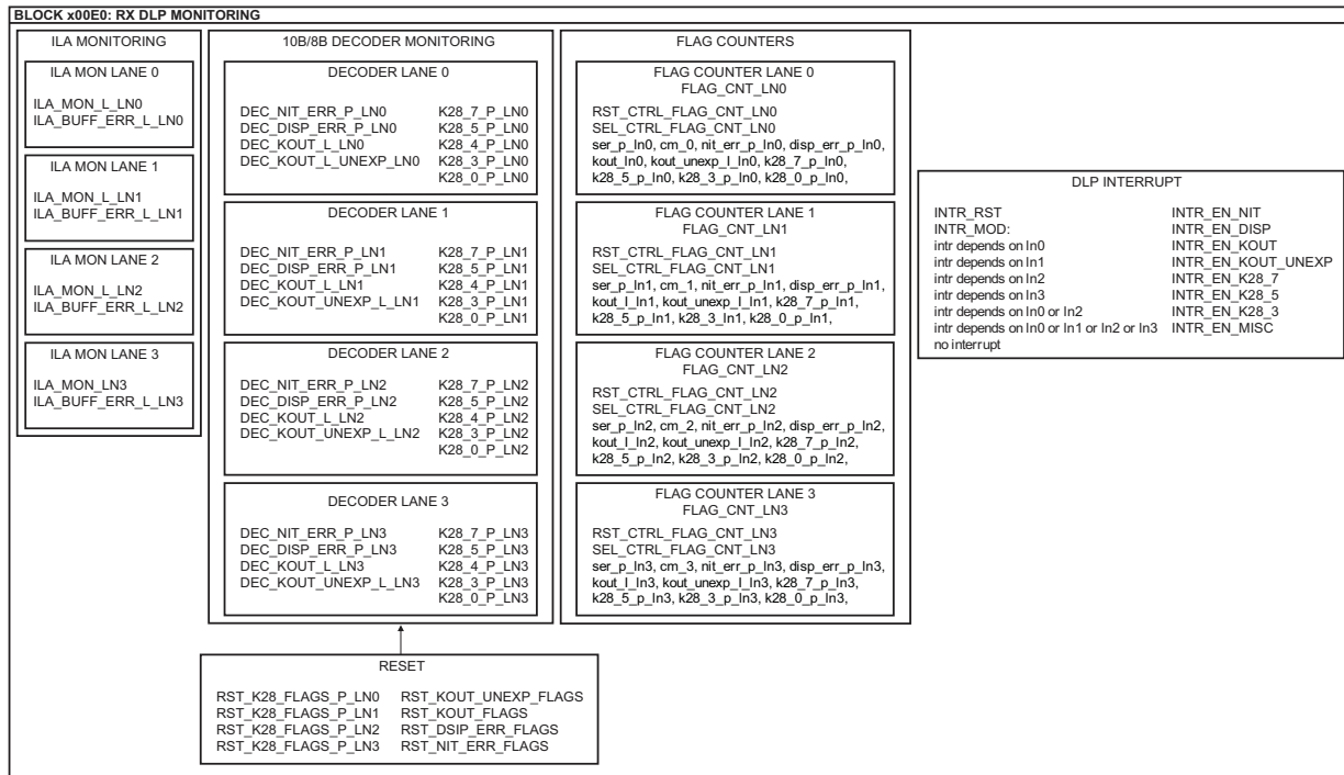
Fig 75. Digital lane processing monitoring
