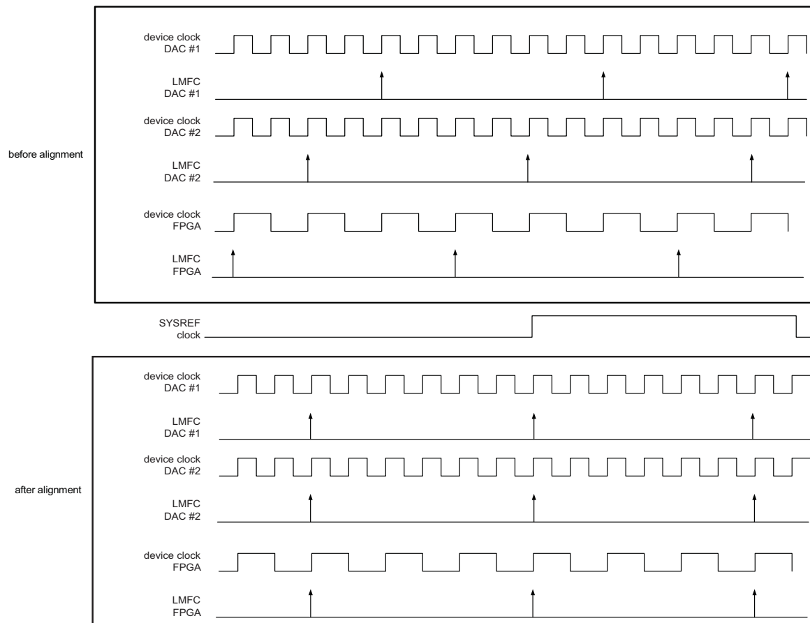
Fig 67. LMFCs before and after alignment to the SYSREF clock
