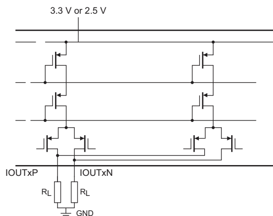
Fig 62. Equivalent analog output circuit
