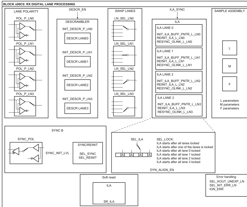
Fig 77. RX digital lane processing
