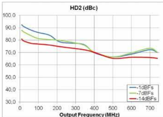
Fig 6. HD2(dBc) over Nyquist depending of f out (MHz) and input level (dBFS)
