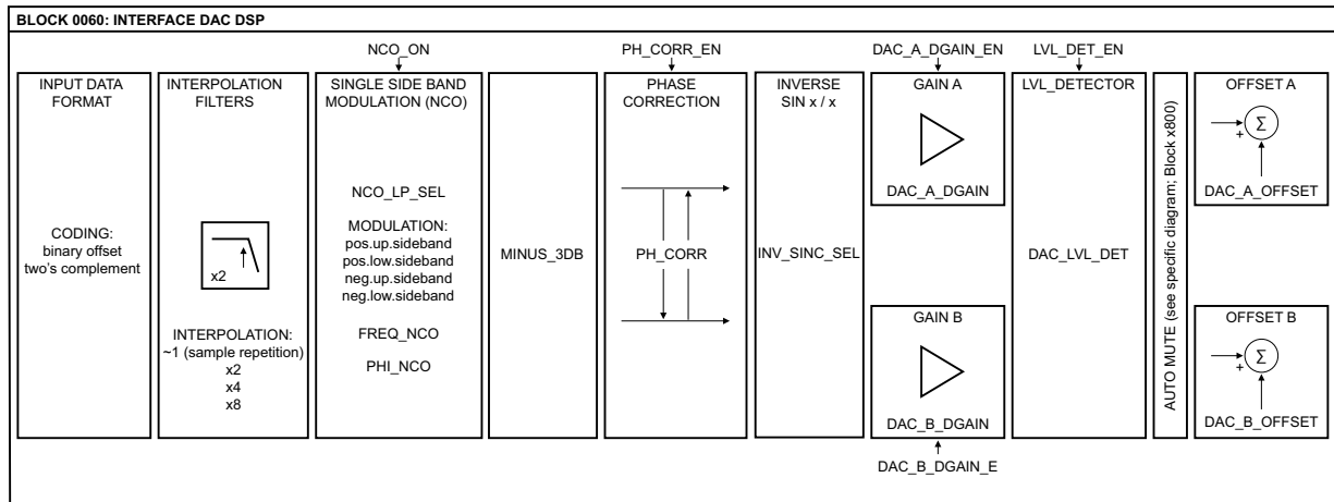
Fig 42. Interface DAC DSP overview
