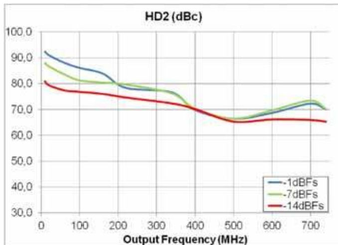
Fig 6. HD2(dBc) over Nyquist depending of f out (MHz) and input level (dBFS)
