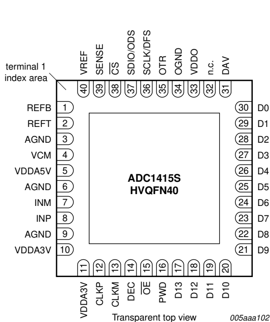
Fig 2. Pin configuration with CMOS digital outputs selected
