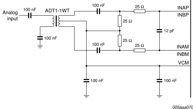
Fig 8. Single transformer configuration
