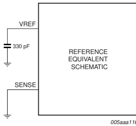
Fig 21. Internal reference, 2 V (p-p) full scale
