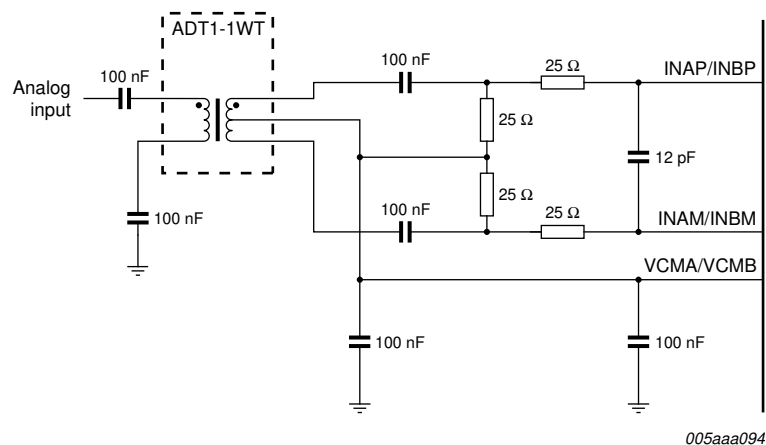
Fig 18. Single transformer configuration suitable for baseband applications
