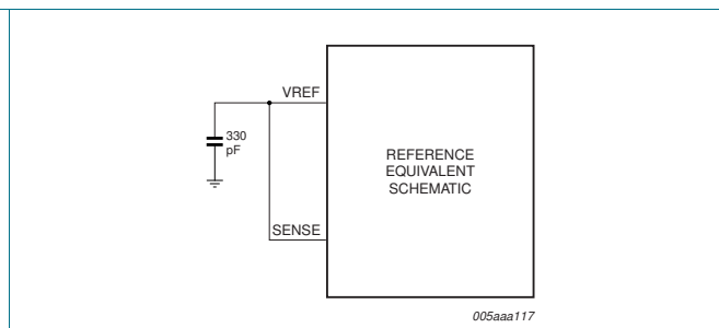
Fig 12. Internal reference, 1 V (p-p) full-scale
