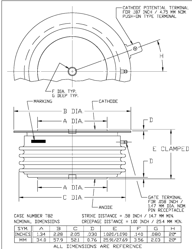
T820 900A (Outline Drawing)
