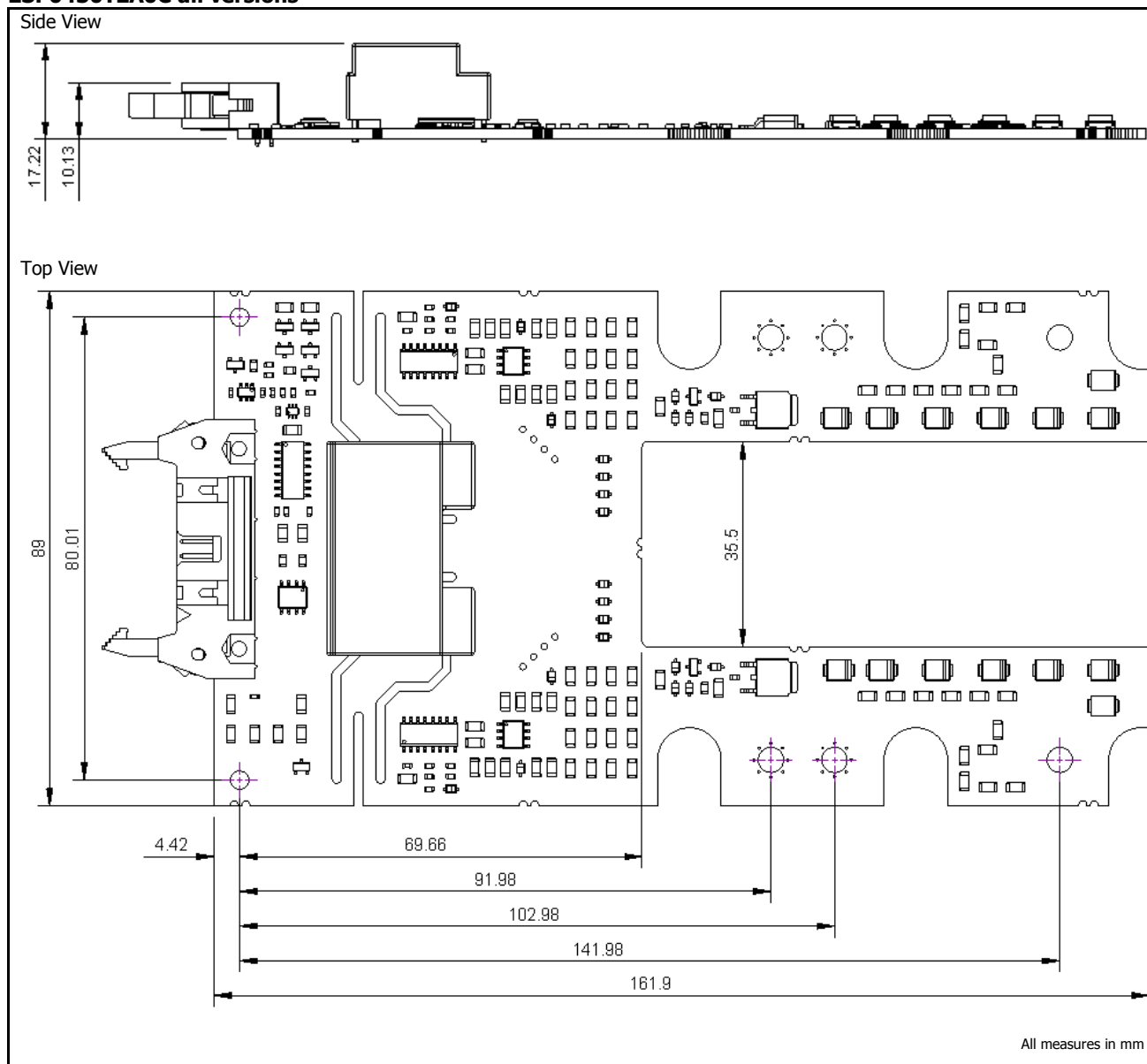
Figure 9. Dimensions.
