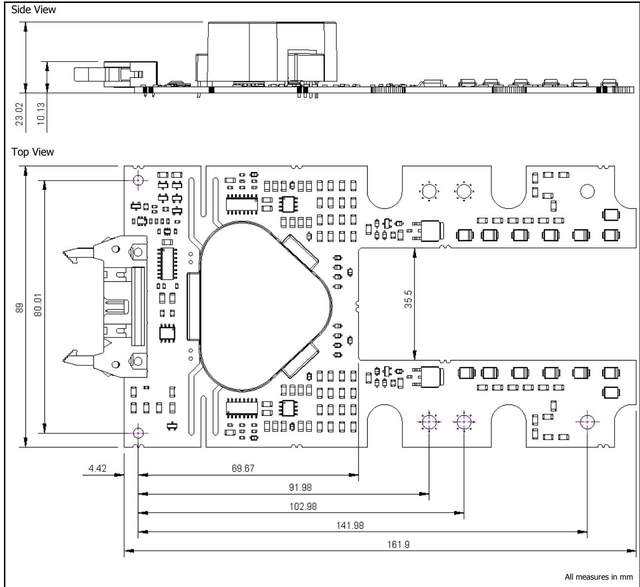
Figure 10. Dimensions.
