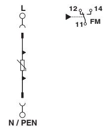
Circuit diagram
