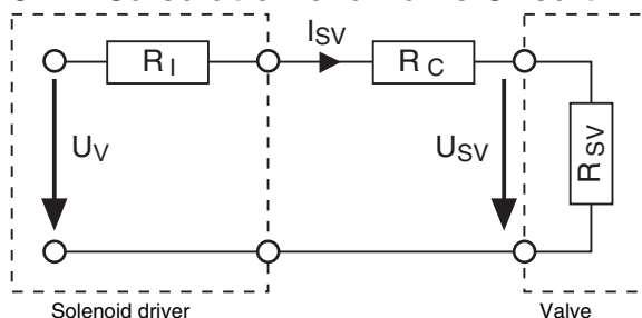
Figure 4 Equivalent circuit
