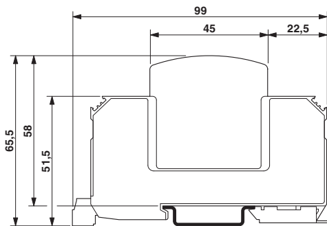
Application drawing
